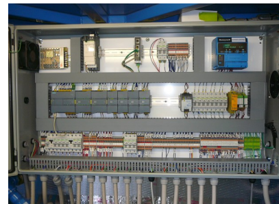
Standard Control Panel with Siemens S7-1200 PLC, automatic circuit breakers, Ethernet Switch, and Honeywell Flame Safeguard.
